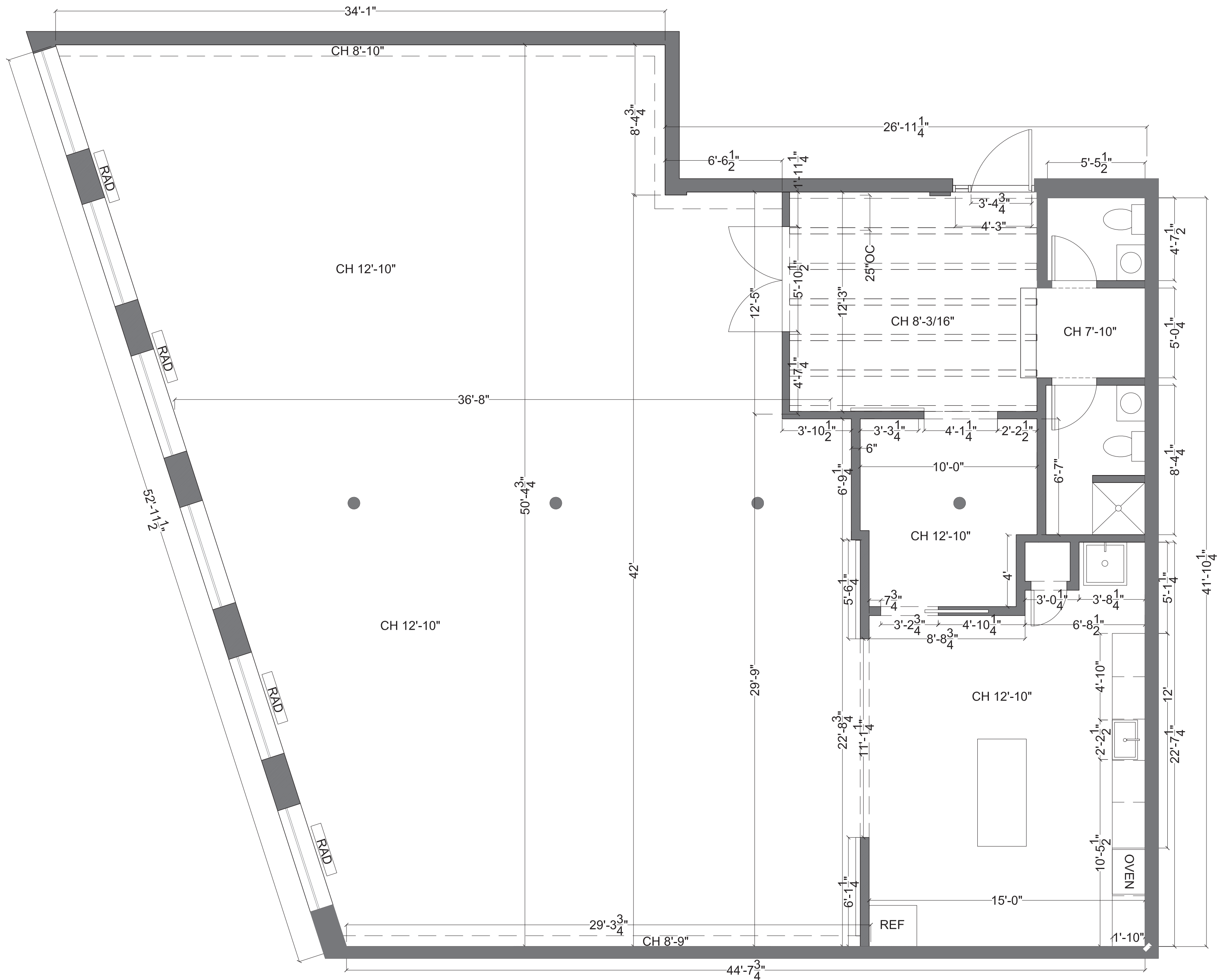
(A) EXISTING PLAN 1/4" = 1'0"
